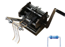
AXIAL IC LEAD CUTTING IC MANUAL FORMING MACHINE
