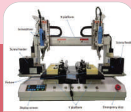
AUTOMATIC SCREW LOCKING MACHINE CUSTOM DESIGN FLOOR TYPE
