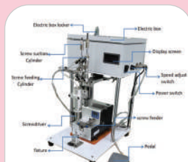
AUTOMATIC SCREW LOCKING MACHINE
